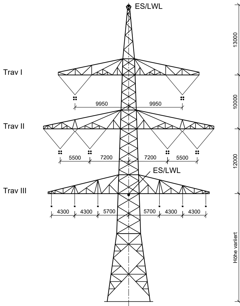
Tragmast T1; DA-4-DE
